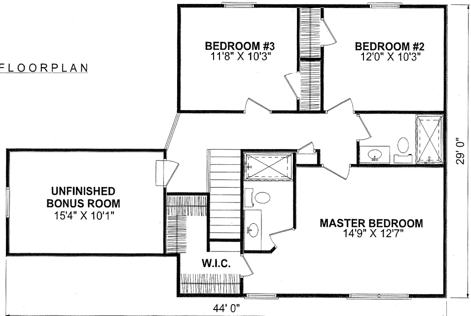
SECOND FLOORPLAN
