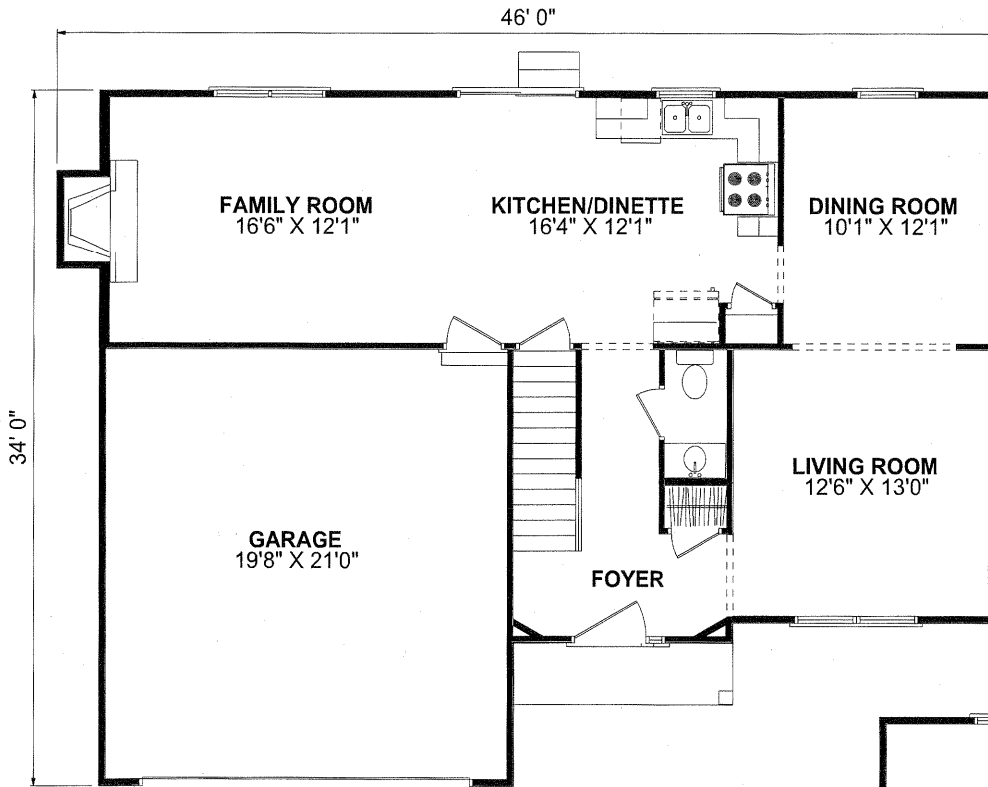
FIRST FLOORPLAN
